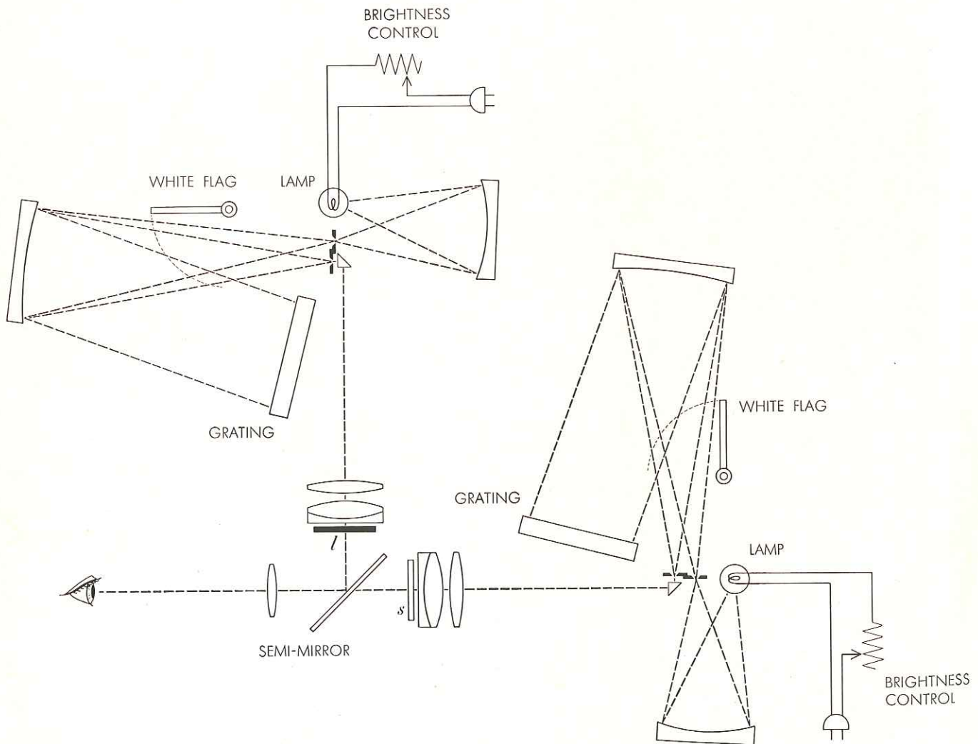
DUAL MONOCHROMATOR used in experiments described in this article is diagrammed. Very narrow bands of wavelengths from any part of the visible spectrum are produced by the two
